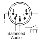
C 0379 5 Pin XLR Wiring Diagram
